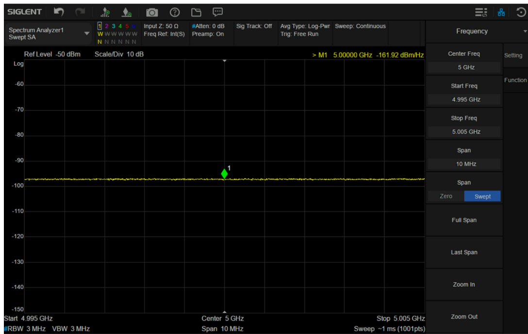
Figure 1-8 Noise power spectral density of analyzer
