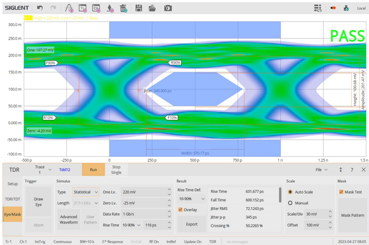
Figure 9: Cable B Passing mask test with injected Jitter
