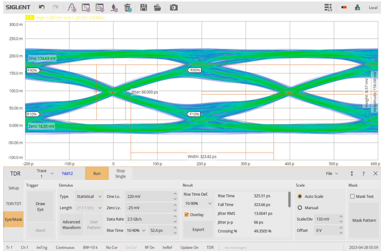
Figure 11: Cable B Operating with a faster edge at 2.5 GB/s
