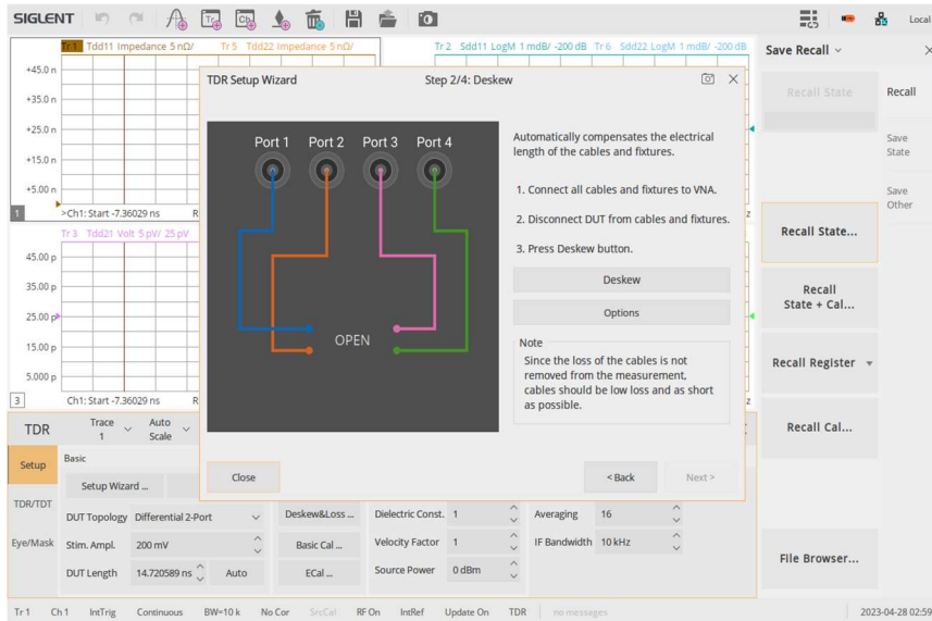
Figure 3: TDR Setup Wizard Deskew calibration
