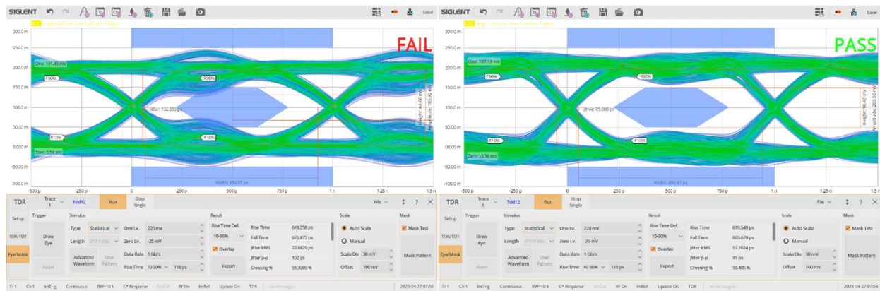
Figure 7: Cable A vs Cable B in Statistical signal simulation with custom Mask
