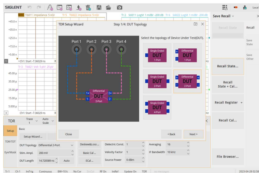
Figure 2: DUT Topology in the TDR Setup Wizard
