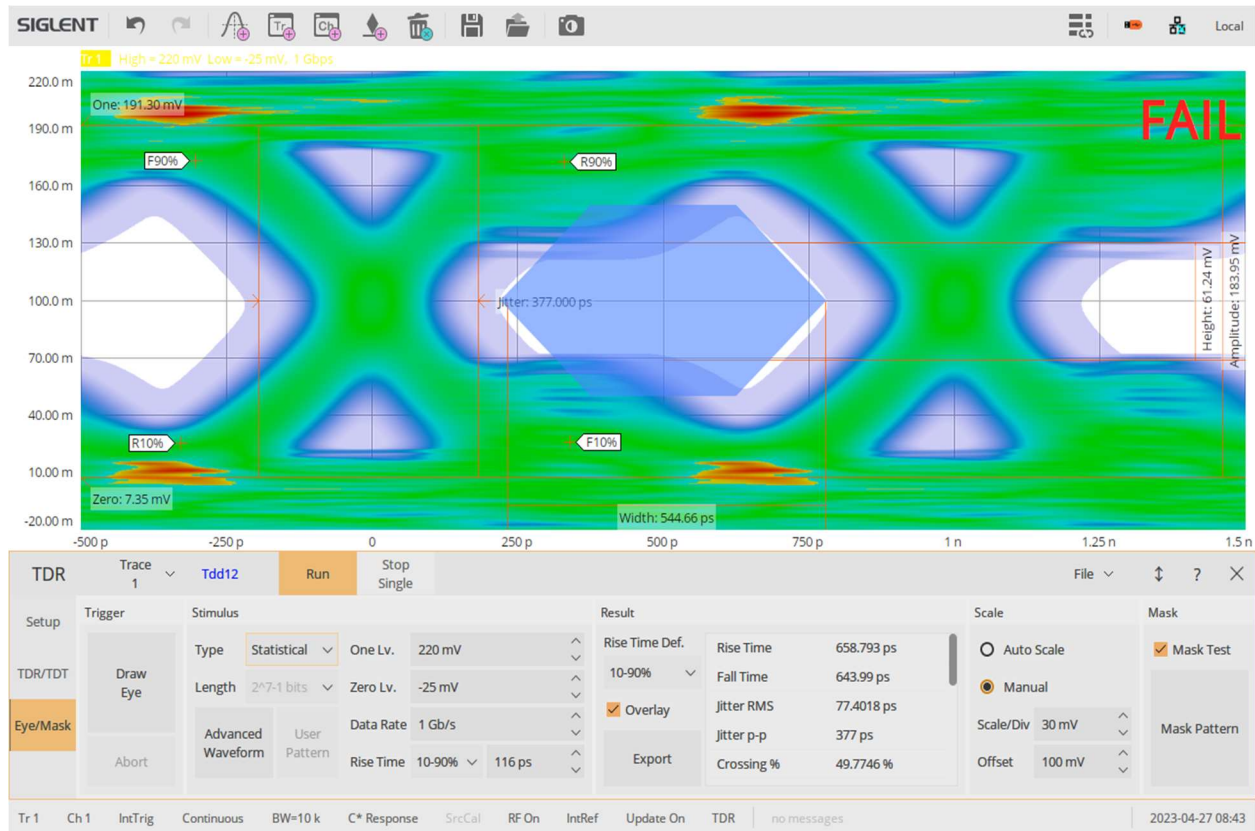
Figure 10: Cable A Failing mask test with injected Jitter
