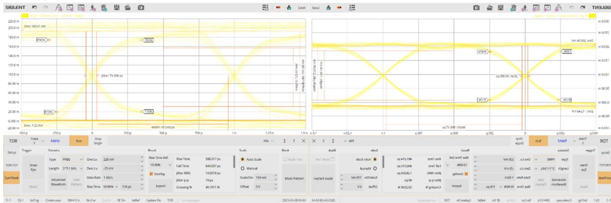
Figure 5: Cable A vs Cable B with PRBS signal simulation
