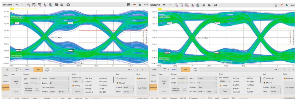
Figure 6: Cable A vs Cable B in Statistical signal simulation
